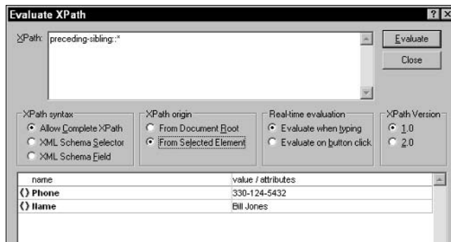
Figure 13-3: Using a selected element in the XPath Analyzer in XMLSpy 2005.
