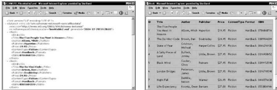
Figure 2-1: An XML file in Internet Explorer.
